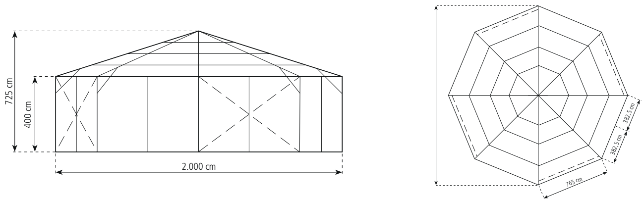
BIG TENT OCTAGONAL 2.000/400/725
