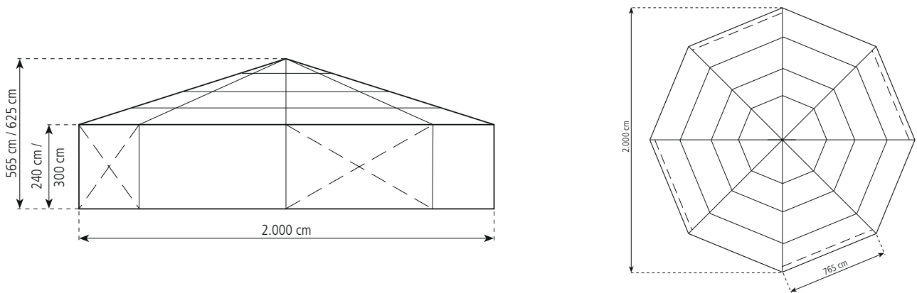
BIG TENT OCTAGONAL 2.000/240/565 & 2.000/300/625
