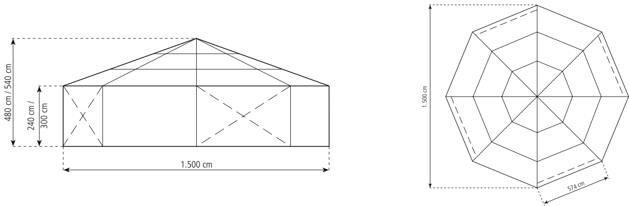
BIG TENT OCTAGONAL 1.500/240/480 & 1.500/300/540
